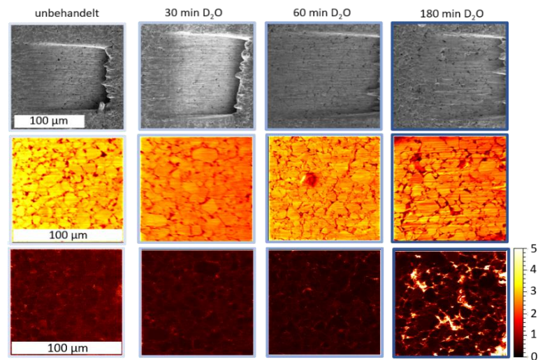
Figure 1: Self Synthesized NCM washed with D 2 O, pressed into Al-Foil, FIB-Cut + ToF-SIMS Analysis
