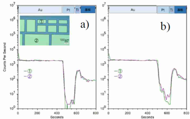
Fig.1 Small area analysis a) Before annealing b) After annealing
