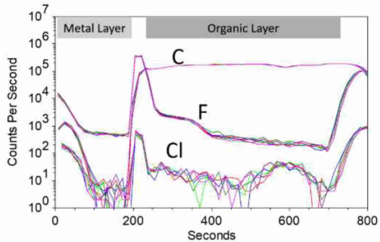
Fig.2 Results of the sample analysis of OLED samples with short lifetime
