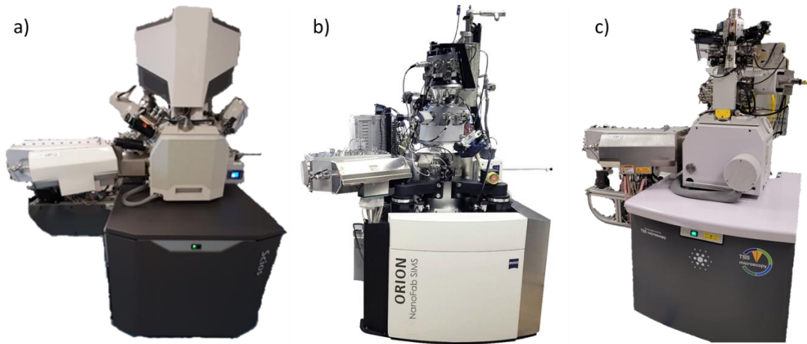
Photos of the Thermo Fisher DualBeam with SIMS, a ZEISS Orion NanoFab Helium Ion Microscope with SIMS and a LoTIS single FIB platform with SIMS. The SIMS add-on system developed at LIST, is mounted on the left side of the FIB and FIB-SEM platforms.
