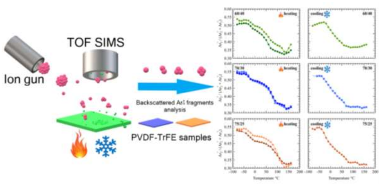
Figure 1. (Left) Principle of the GCISS measurement. (Right) Temperature dependence of the Ar_2^+ / (Ar_2^+ + Ar_3^+) breaking ratio upon heating and cooling of P(VDF- ran -TrFE) thin films. The continuous lines are interpolated smoothing splines.
