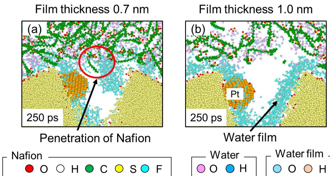
Fig. 2 Coverage state of Nafion over the Pt nanoparticle in the interior of the pore when the thickness of water film is (a) 0.7 and (b) 1.0 nm, respectively.
