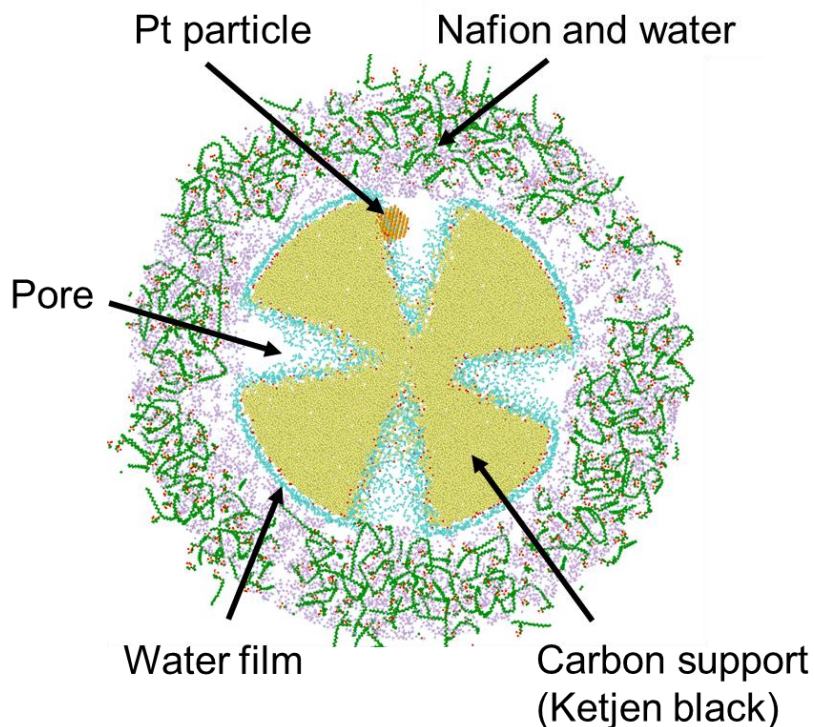
Fig. 1 Cross-sectional view of CP model
