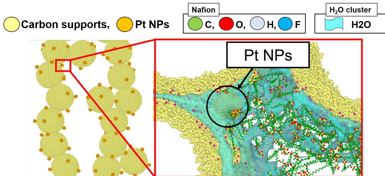
Fig. 3 Overall view of carbon supports and magnified view of Nafion coverage on Pt NPs surrounded by three carbon carriers
