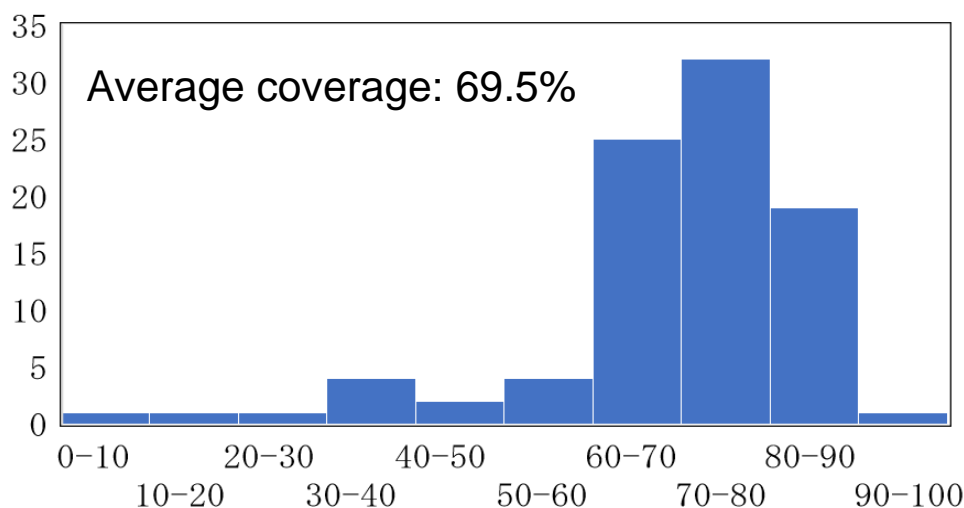
Fig. 2 Distribution of Nafion coverage on each Pt NPs
