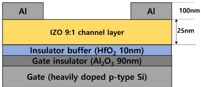
Fig. 1. Cross-sectional schematic diagram of IZO TFTs with HfO 2 /Al 2 O 3 gate insulator.
