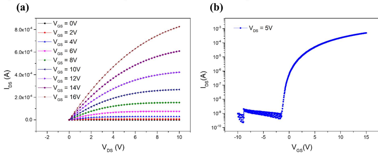
Fig. 2. (a) Output curves and (b) transfer curves of IZO TFTs with HfO 2 /Al 2 O 3 gate insulator.
