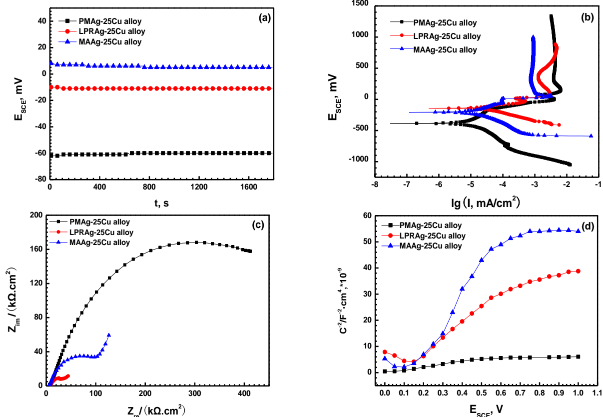
Fig. 3 Open Circuit potential (a), polarization (b), EIS (c), and Mott-Schottky (d) curves of three Ag-25Cu alloys in NaCl neutral solutions.
