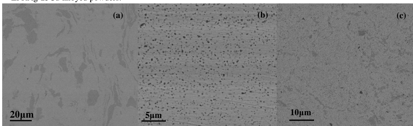
Fig. 2 Microstructures of PMAg-25Cu (a), LPRAg-25Cu (b) and MAAG-25Cu (c) alloys
