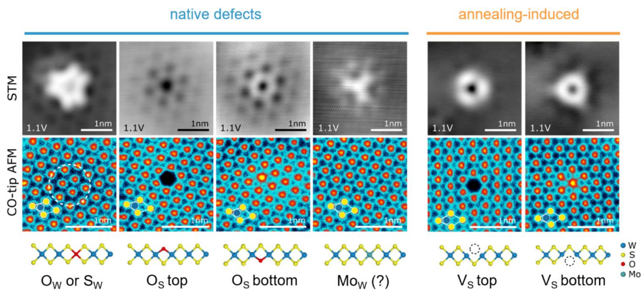
Fig 1. First row: STM topography of different point defects of CVD-grown monolayer WS_2 on multilayer graphene on SiC. Second row: CO-tip AFM images of the same defects with the unit cell of WS_2 indicated.
