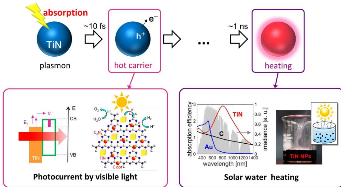
Fig. 1. Schematic of optically excited TiN nanostructures and associated photoelectric and photothermal conversions for hot electron generation and solar water heating, respectively.
