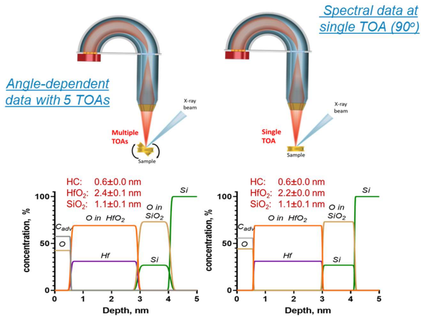
Figure 2. StrataPHI layer thickness calculation – 5 TOAs vs single TOA.
