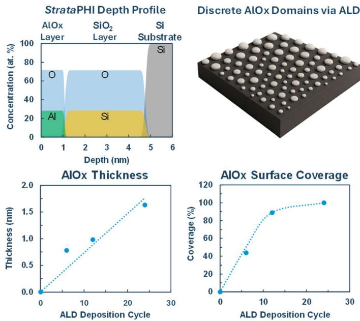
Figure 1. Non-destructive fractional coverage and layer thickness calculation by StrataPHI .
