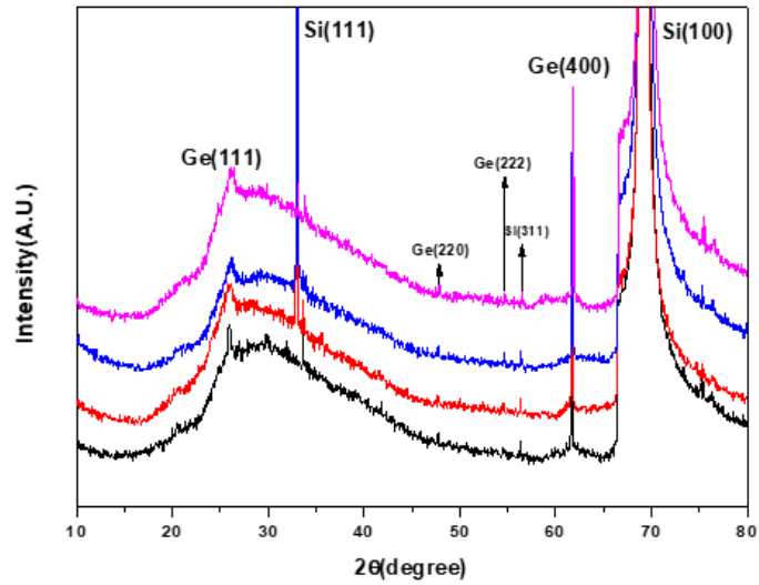
Figure 2. The XRD of DC sputter deposited Ge films
