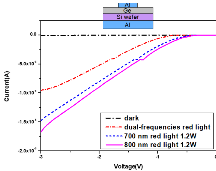
Figure 2. The I-V characteristics of Ge/Si junction under various illuminations
