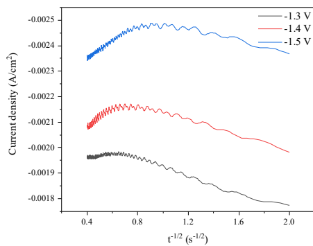
Figure 2. Cottrell curves for the Co(P) film
