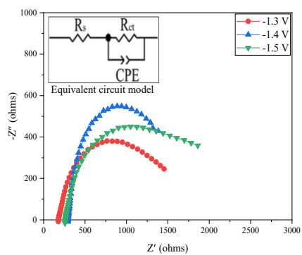
Figure 1. EIS results of the Co(P) films
