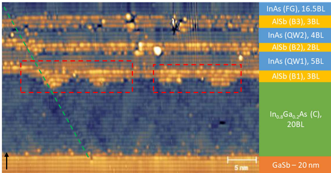
Figure 1. 40 \times 35 nm filled state topography image of the TBRT structure, the InGaAs layer and the GaSb layer ( V_b = -3 V and I_t = 50 pA). The QPs and the slip plane are highlighted by the dashed red rectangles and the dashed green line, respectively. The arrow indicates the growth direction. BL: atomic bilayers, i.e. lattice constants.
