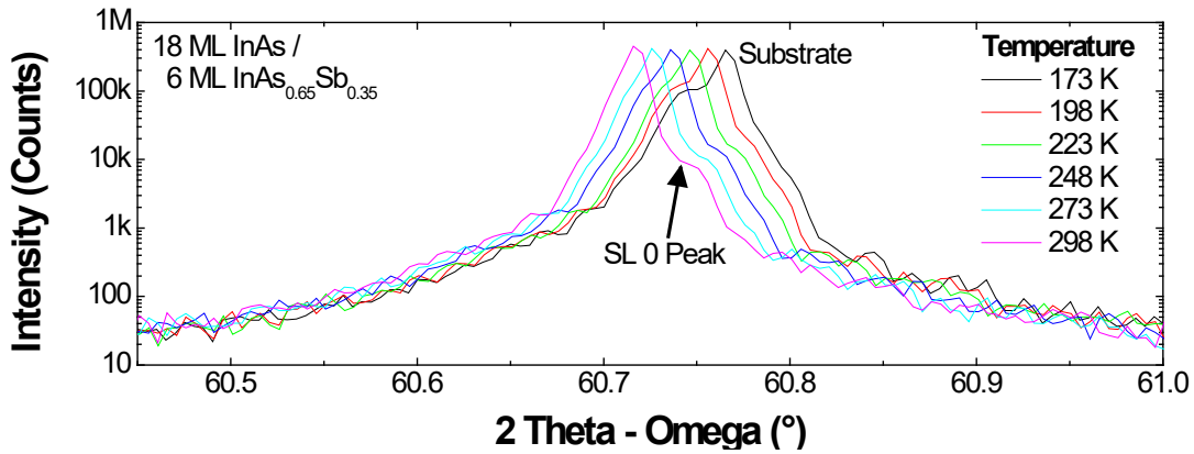
Evolution of SL0 and substrate peak with temperature for two different strained-layer superlattices. C. J. Reyner, et al Crystals 6(1) 2016 p150
