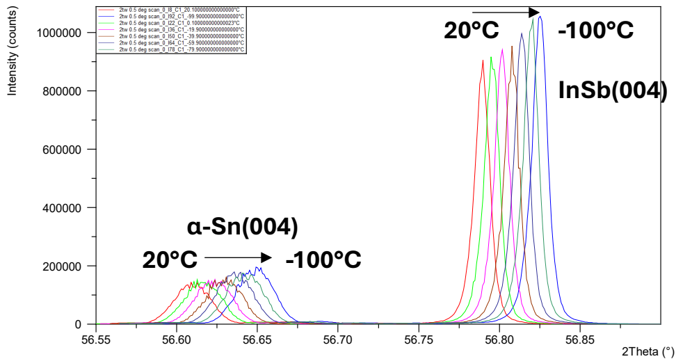
Evolution of film and substrate peaks for \alpha -Sn/InSb(001).
