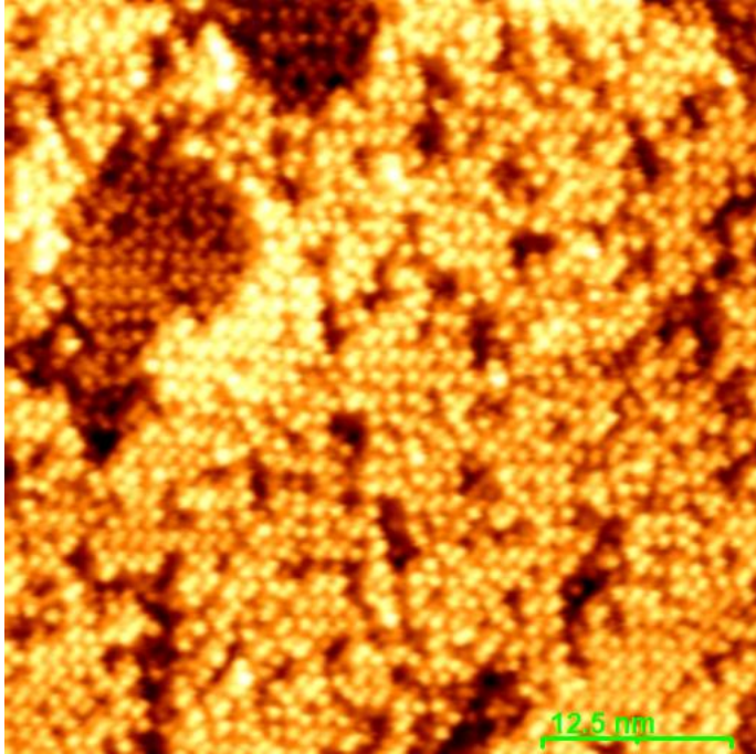
Figure 1: STM image showing long range order of 3D Sn growth of Sn on Si, >1 ML.
