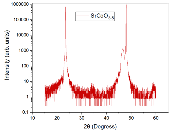
Fig 3: XRD analysis of SCO film grown on LAO
