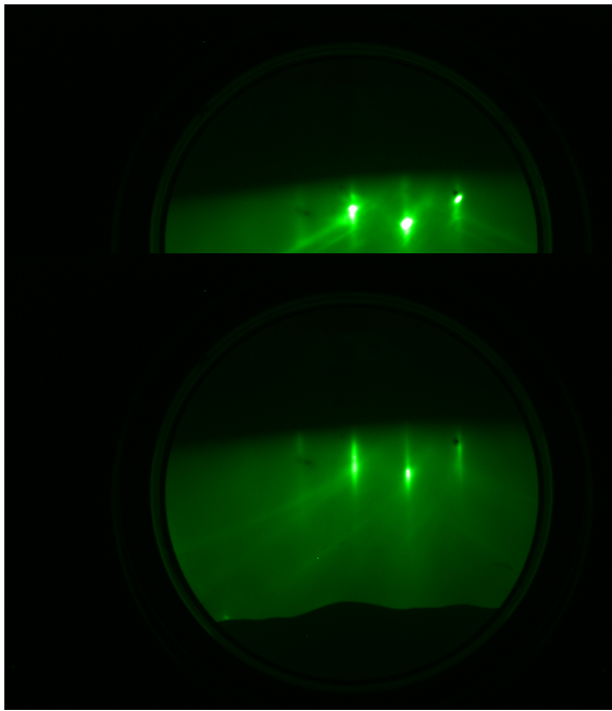
Fig 1: \text{LaAlO}_3 (LAO) substrate before growth (top), \text{SrCoO}_x (SCO) film grown on LAO (bottom)
