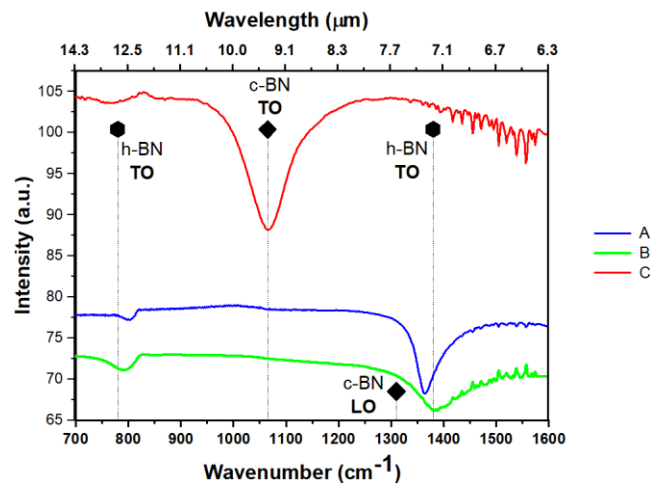
Figure 1: FTIR spectra of BN films grown under a Mg flux (A), an Ar ion flux (B), and both Mg and Ar ion fluxes (C). Only spectrum C is characteristic of c-BN.
