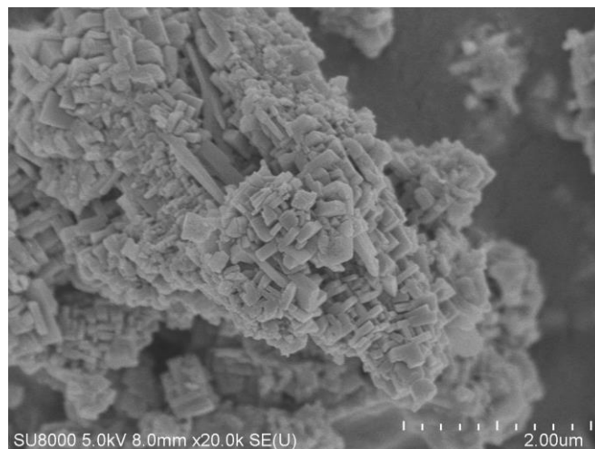
Fig. 3 Cross-stacking thick plate-like \text{NaNbO}_3 fabricated using 60 mM \text{Nb}_2\text{O}_5 , 12 M NaOH, and annealed at 160 °C for 12 h.
