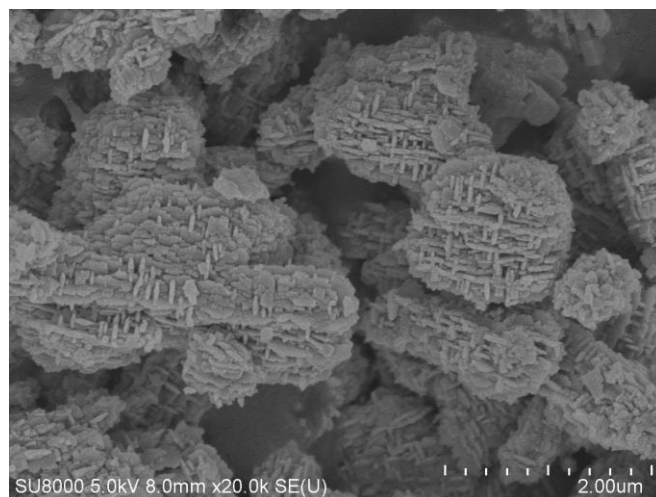
Fig. 2 Cross-stacking thin plate-like \text{NaNbO}_3 fabricated using 60 mM \text{Nb}_2\text{O}_5 , 12 M NaOH, and annealed at 160 °C for 4 h.
