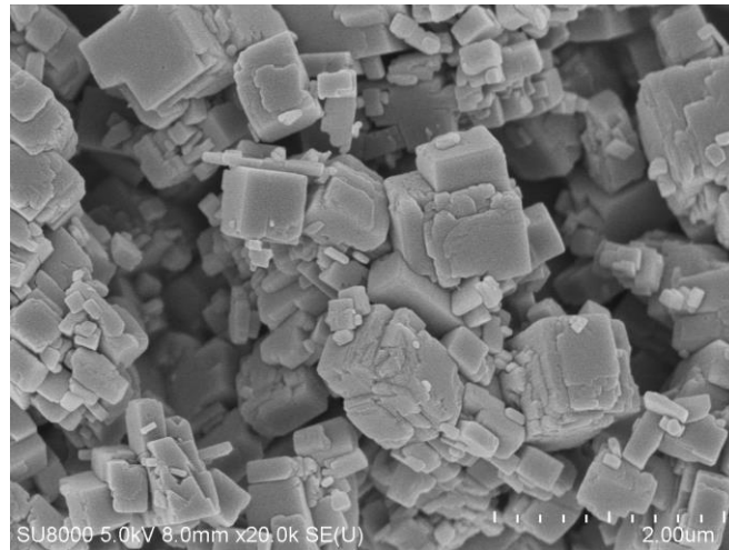
Fig. 1 Cubic-like \text{NaNbO}_3 fabricated using 30 mM \text{Nb}_2\text{O}_5 , 3 M NaOH, and annealed at 150 °C for 48 h.
