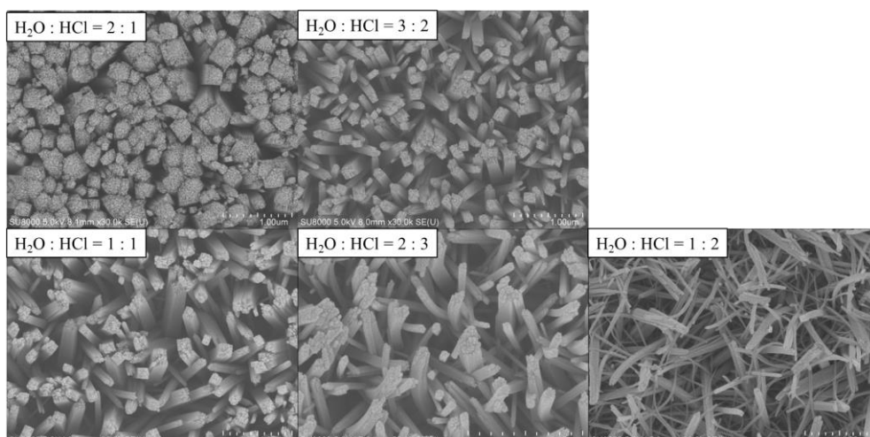
Fig. 2 Top view of SEM graphs of the morphology-tuning of \text{TiO}_2 template.
