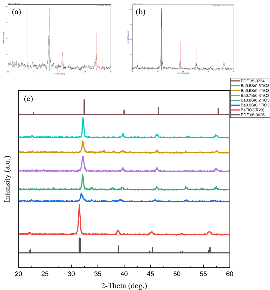
Fig. 1 XRD diagram of (a) \text{TiO}_2 (b) \text{BaTiO}_3 (c) (\text{Ba,Sr})\text{TiO}_3 nanorod arrays.
