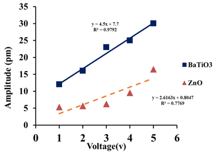
Fig. 3. The piezoresponse of BaTiO 3 nanorod arrays measured under different bias from PFM.
