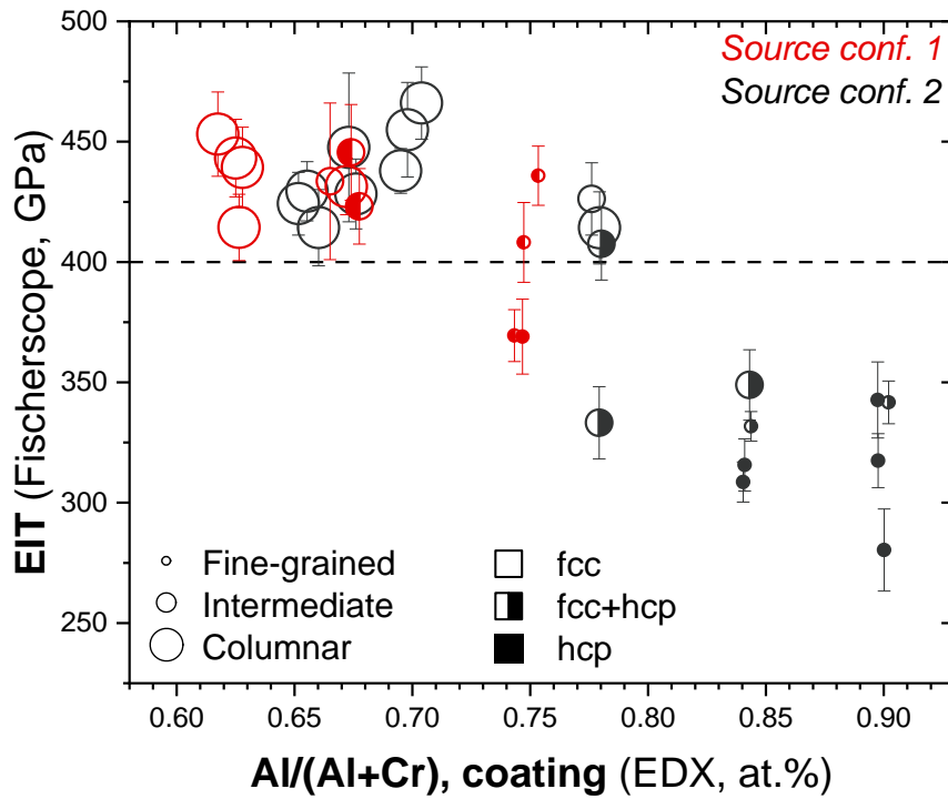
Effect of the arc source configuration (conf. 1 and conf. 2) on the evolution at room temperature of the Young's modulus EIT, morphology (columnar, intermediate and fine-grained) and crystal structure (fcc, fcc+hcp and hcp) of AlCrN films deposited by cathodic arc with an increasing Al content.
