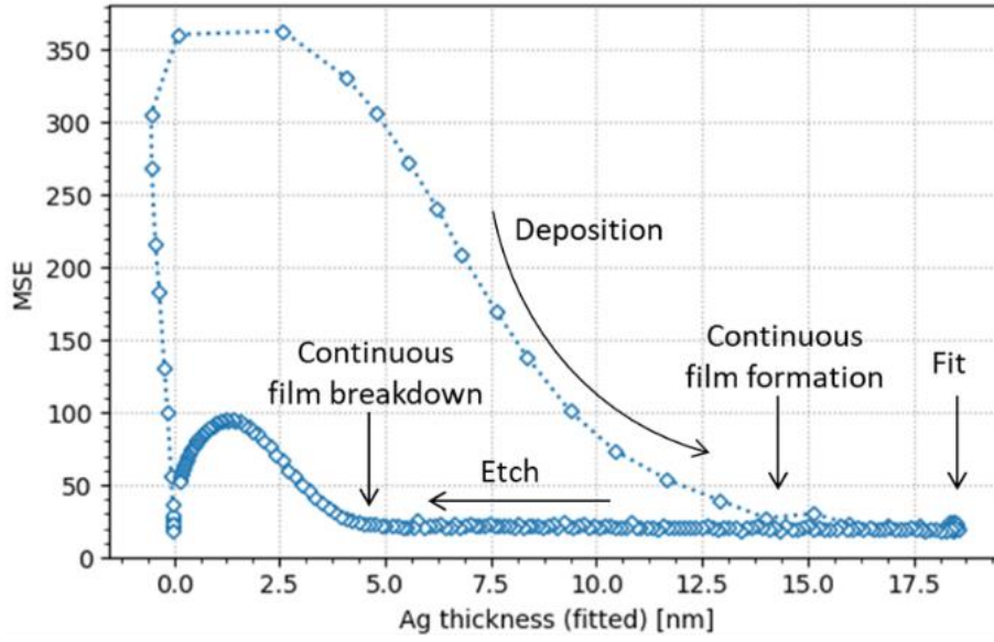
Figure 1: Example of in-situ film coalescence monitoring: mean square error plotted versus the Ag film thickness.
