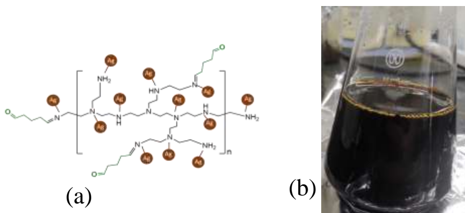
Fig. 1 catalyst : PEI-GA-Ag (a) structure and (b) sample
