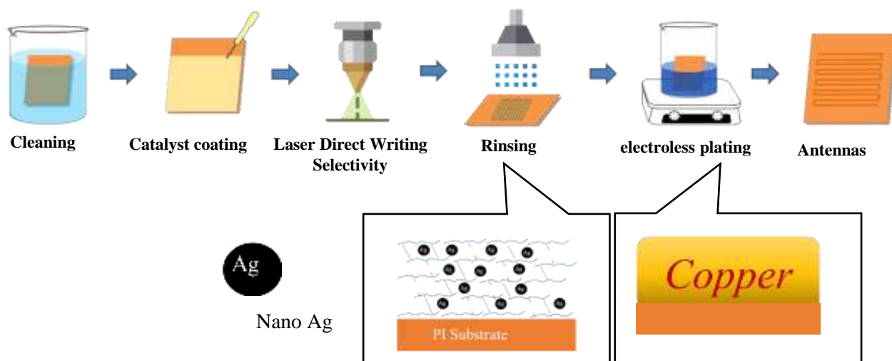
Fig. 2. Scheme for manufacturing copper Antennas patterns on PI surface
