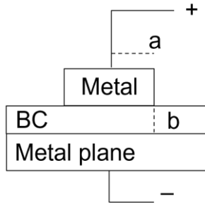
Figure 1 Boron carbide resistor schematic
