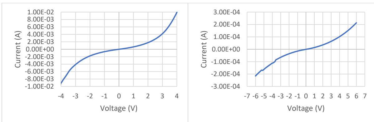
Figure 2 Ti-BC(n)-Ti Schottky contact I-V curve (left), Cr-BC(n)-Cr Schottky contact I-V curve (right)
