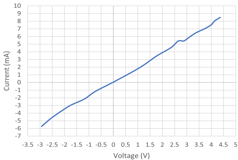
Figure 3 Cr-BC(p)-Cr Ohmic contact I-V curve
