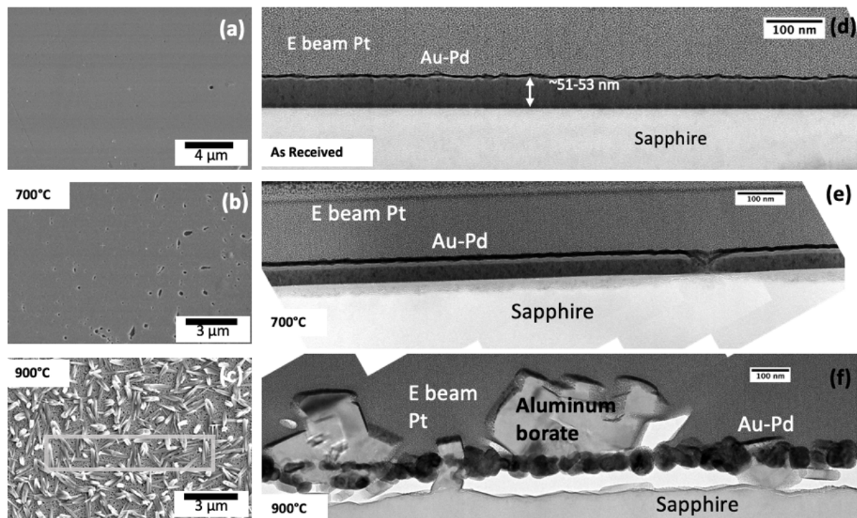
Fig 1: (a), (b), and (c) are top view scanning electron micrographs; (d), (e), and (f) are cross sectional transmission electron micrographs. (a) and (d), prior to heat treatment; (b) and (e), after annealing at 700°C; (c) and (f), after annealing at 900°C.
