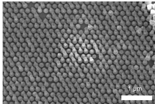
Figure 2. SEM image of the nanostructures of the GLAD features
