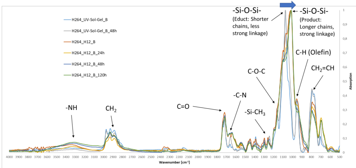
Figure 2: FTIR-Study on the hardening process of the sol-gel
