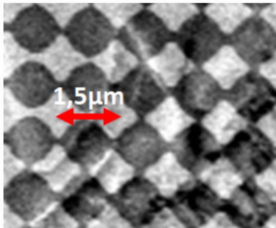
Figure 2: Detail of the gold grid pattern for DIC
