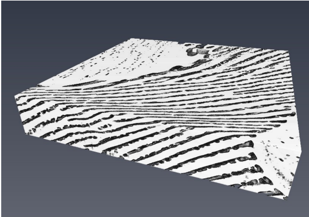
Figure 1: 3D reconstruction of the microstructure of Zn-Al coating
