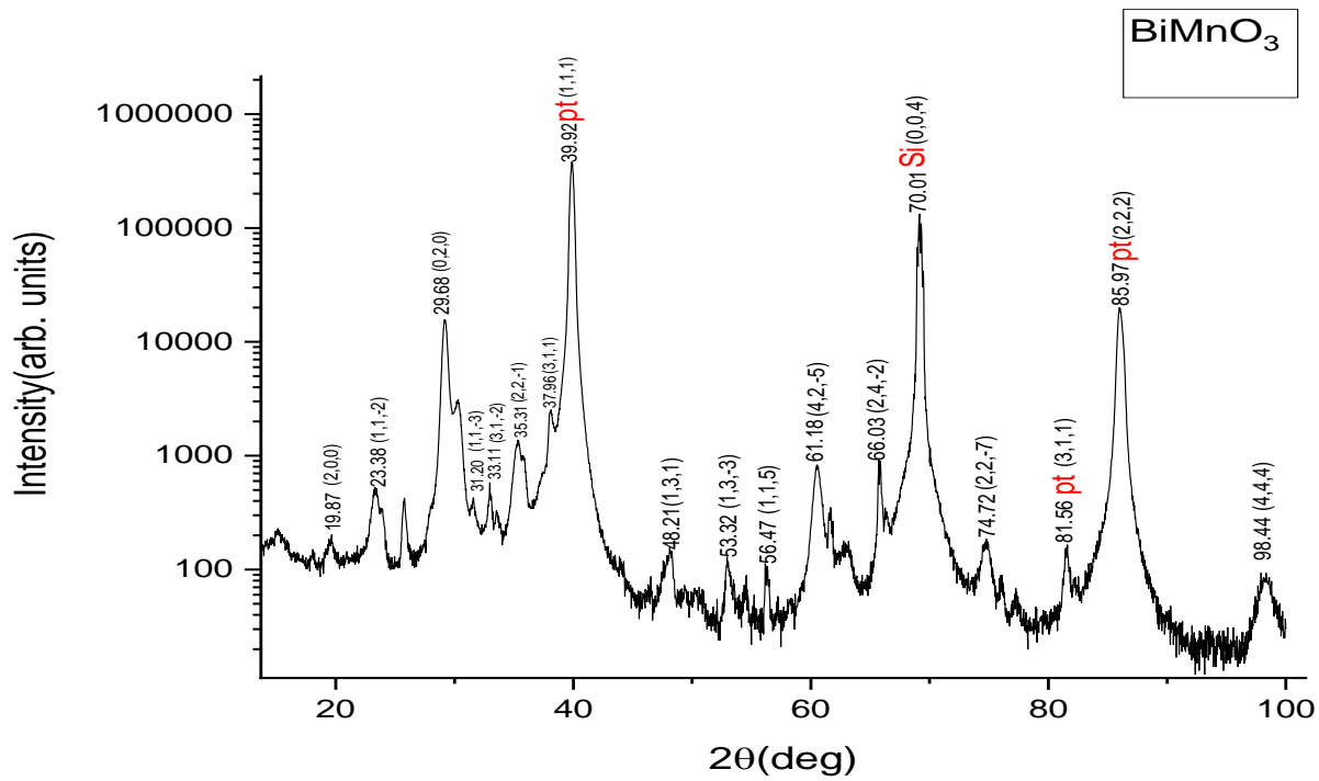
XRD patterns of BiMnO 3 thin films grown on SiO 2 /TiO 2 /Pt (111) substrates
