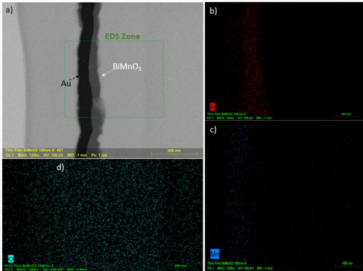
EDS map distribution of the elements of a BiMnO 3 thin film.
