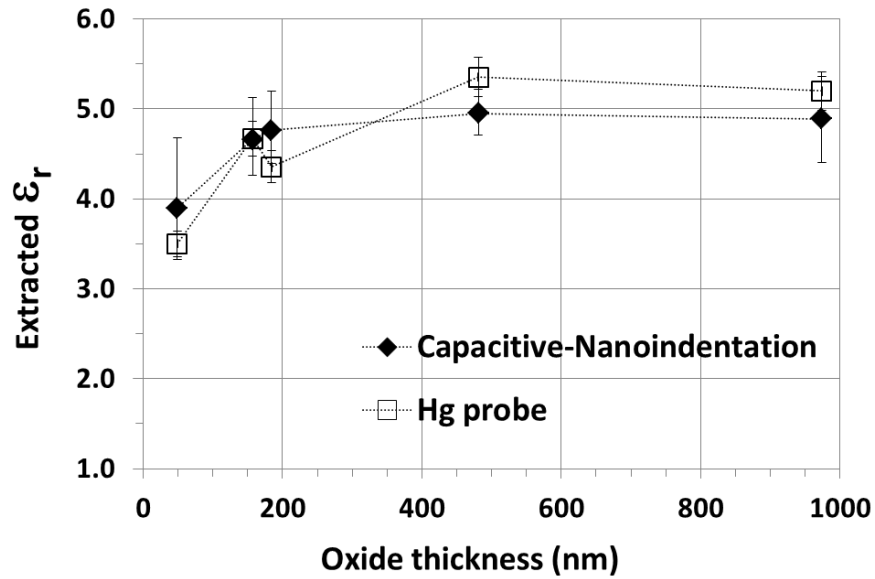
Figure 1: Local measurements of dielectric permittivity on different silica films (compared to macroscopic Hg-probe measurements).
