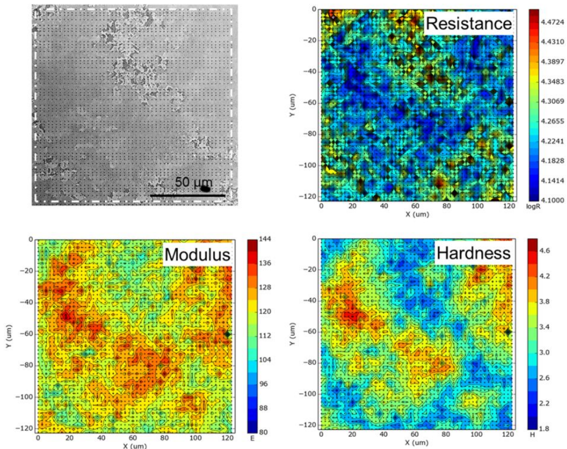
Figure 2: SEM micrograph and the corresponding electrical/mechanical properties of a multiphased metallic alloy.
