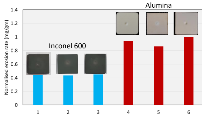
Figure 2. 1000 °C erosion rates for IN600 and alumina
