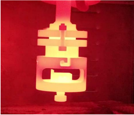
Figure 1. 1000 °C sample mounted in erosion holder
