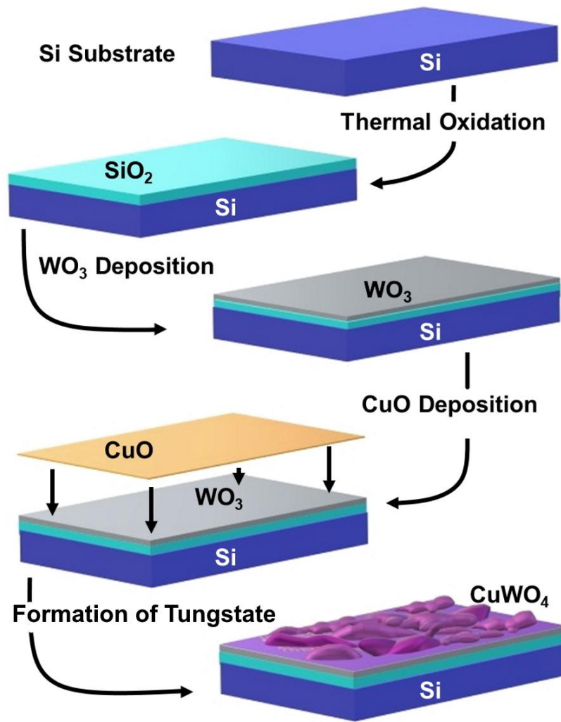
Figure 1 Schematic of process of preparing nanostructured \text{CuWO}_4/\text{WO}_3 bilayers.
