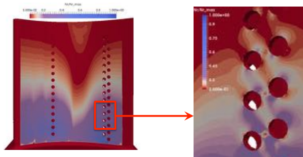
Fig. 2 Lifetime modeling of a turbine blade (courtesy of B. Marchand)
