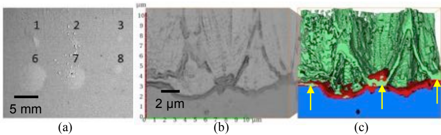
Fig. 1 Specimen after LASAT (a) top-view evidencing the contrast induced by debonding (b) FIB BSE and (c) segmented images : bond-coat in blue, TGO in red, gaps between columns and crack in green and yellow arrows indicating micro-cracks within, below and above the oxide layer [4]
