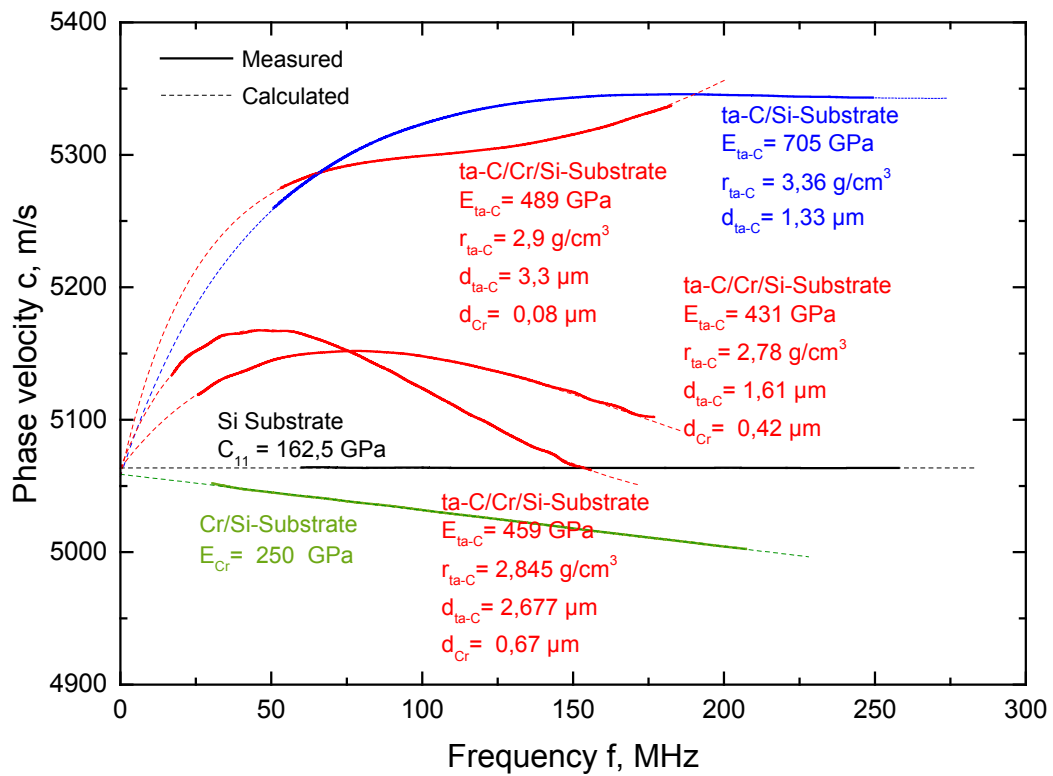
Figure 1: Measured and calculated dispersion curves for the coating systems Si substrate uncoated (black), Cr/Si (green), ta-C/Si (blue) and several variants of ta-C/Cr/Si (red) and the correspondingly calculated material properties
