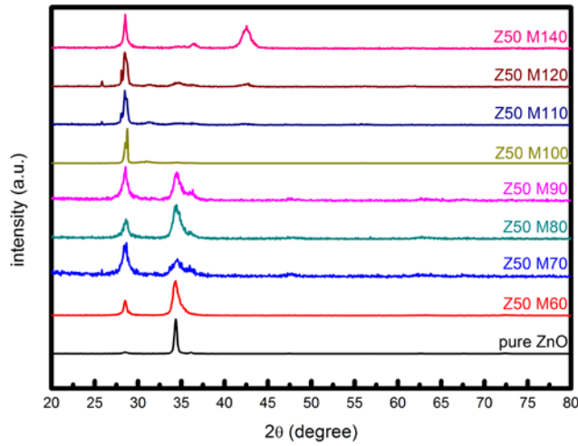
Figure 2. XRD plot of films with different Mg content.
