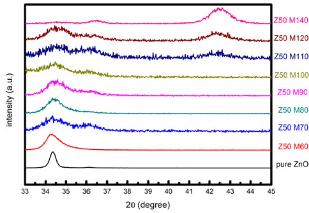
Figure 1. Slow scan of XRD plot of films with different Mg content.
