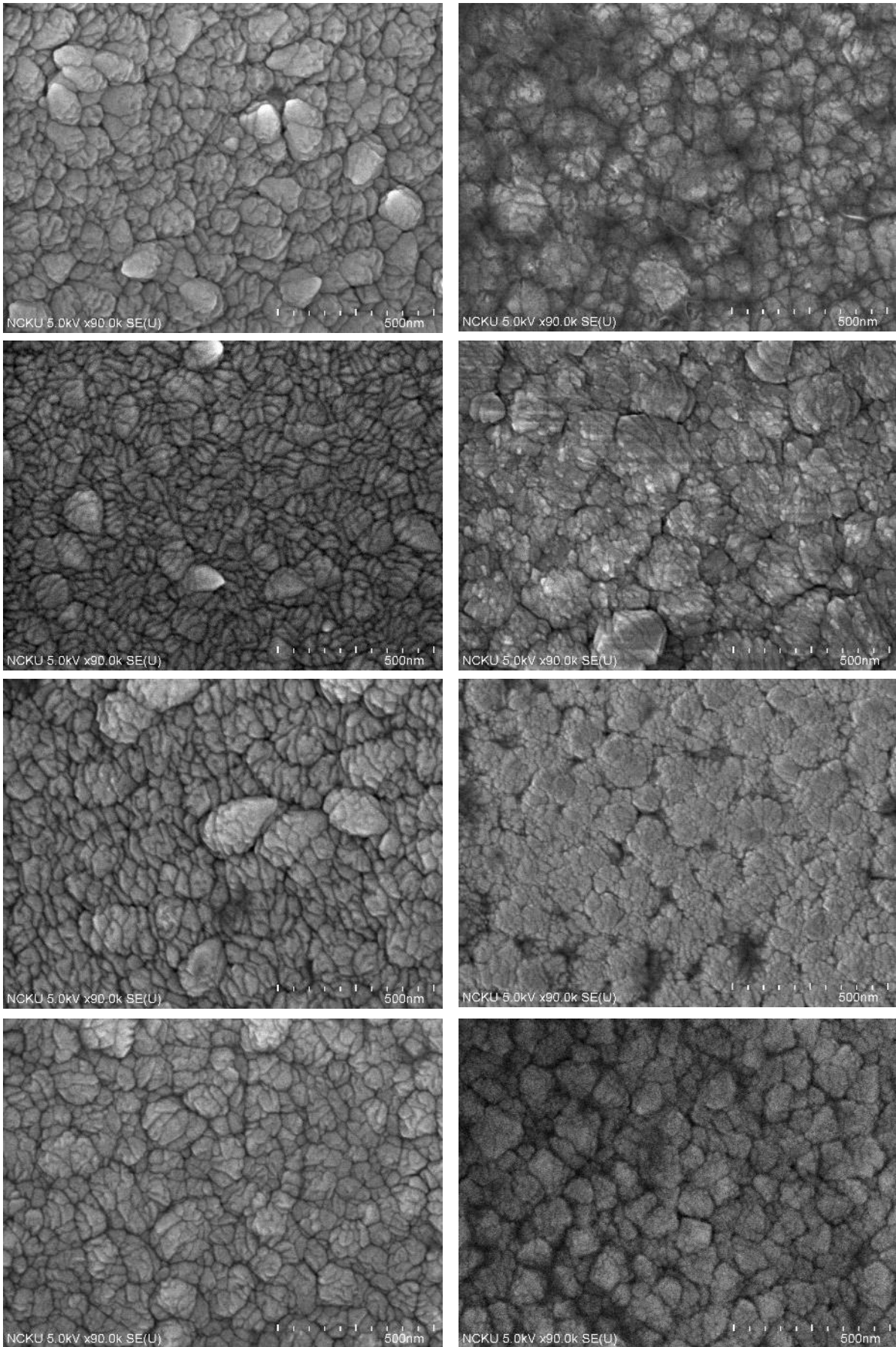
Figure 4. The topview images of SEM of films with different Mg compositions. (From top to bottom: lefts are Mg content of 5.46at%, 8.23at%, 10.54at%, and 11.43at%; rights are Mg content of 13.59at%, 15.57at%, 18.81at%, and 19.76at%.)
