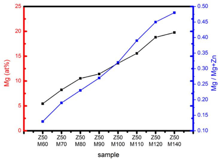
Figure 3. EDX results of films with different Mg content.
