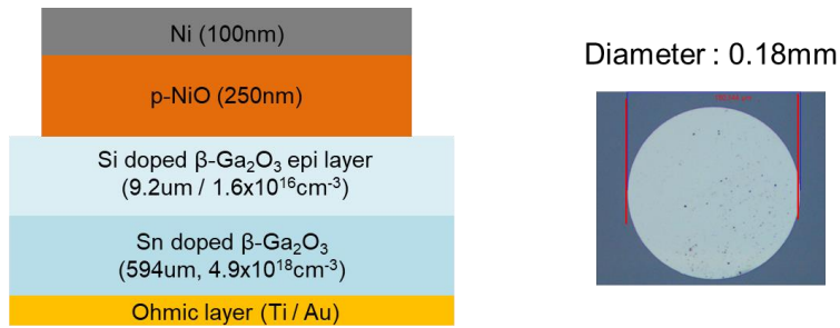
Fig.1. Schematics of vertical pn heterojunction diode
