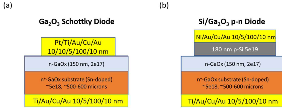
Figure 1. Device structure of the (a) Ga 2 O 3 Schottky diode and (b) p-Si/n-Ga 2 O 3 diode.
