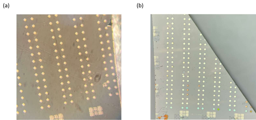
Figure 2. Optical image of the (a) Ga 2 O 3 Schottky diodes and (b) p-Si/n-Ga 2 O 3 diodes.
