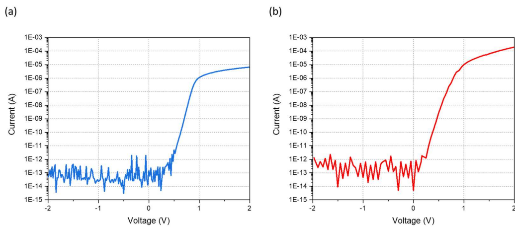
Figure 3. I-V characteristic of the (a) n-Ga 2 O 3 Schottky diode and (b) p-Si/n-Ga 2 O 3 diode.
