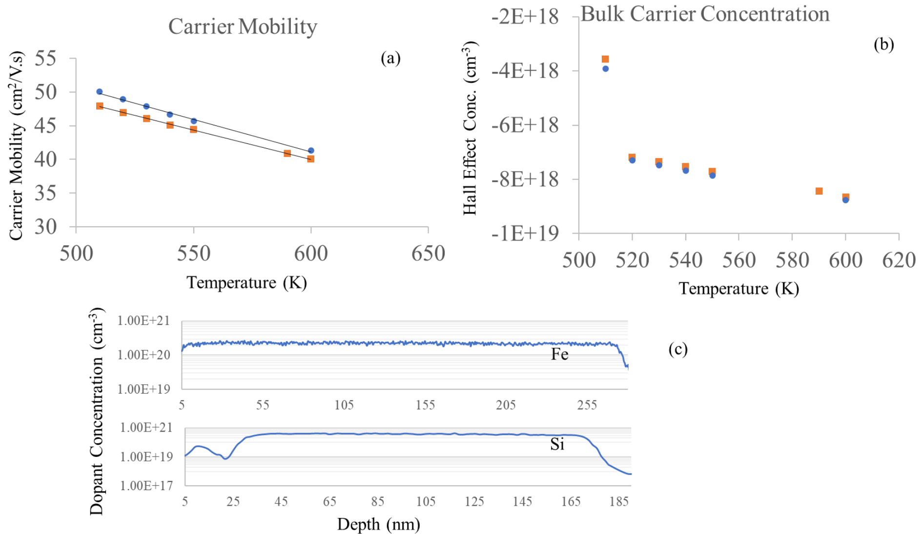
Figure: (a) Carrier mobility from Hall Effect data at elevated temperature, (b) Bulk carrier concentration from Hall Effect, (c) Dopant concentration from SIMS data.
