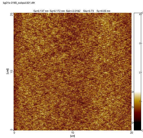
Figure 3: AFM Scan Showing Consistent Surface
