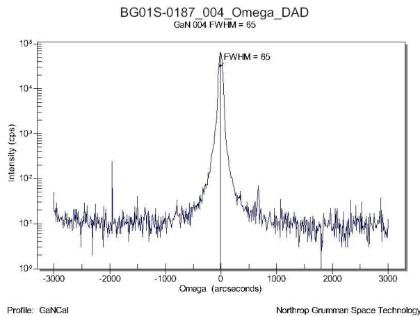
Figure 4: XRD Scans showing FWHM of (020) of 65 arc sec.
