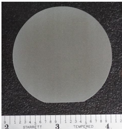
Figure 2: 2" \beta -Ga 2 O 3 wafer with (100) orientation flat.
