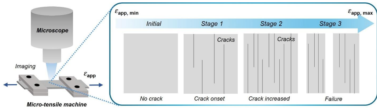
Figure 1. Schematic illustration of the in situ mechanical testing setup for quantifying the elastic modulus, crack onset strain, crack density, fracture toughness, and interfacial shear strength of ALD-coated films.
