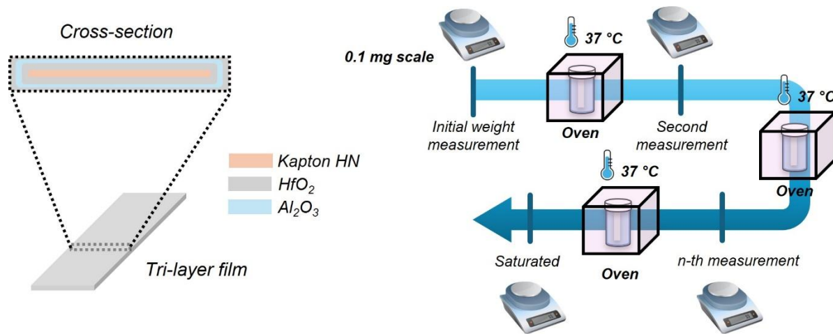
Figure 2. Schematic illustration of the tri-layer coated film, its cross-sectional structure, and the sorption testing method in DI water under physiological temperature (37°C).
