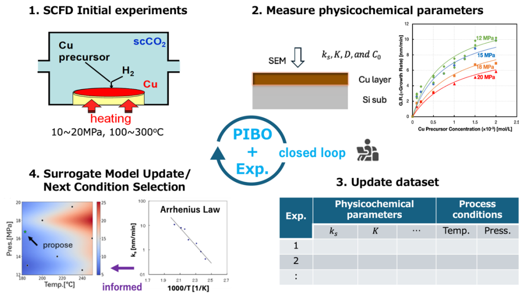
fig 2. Closed-Loop Workflow of the Proposed SCFD Optimization Framework
