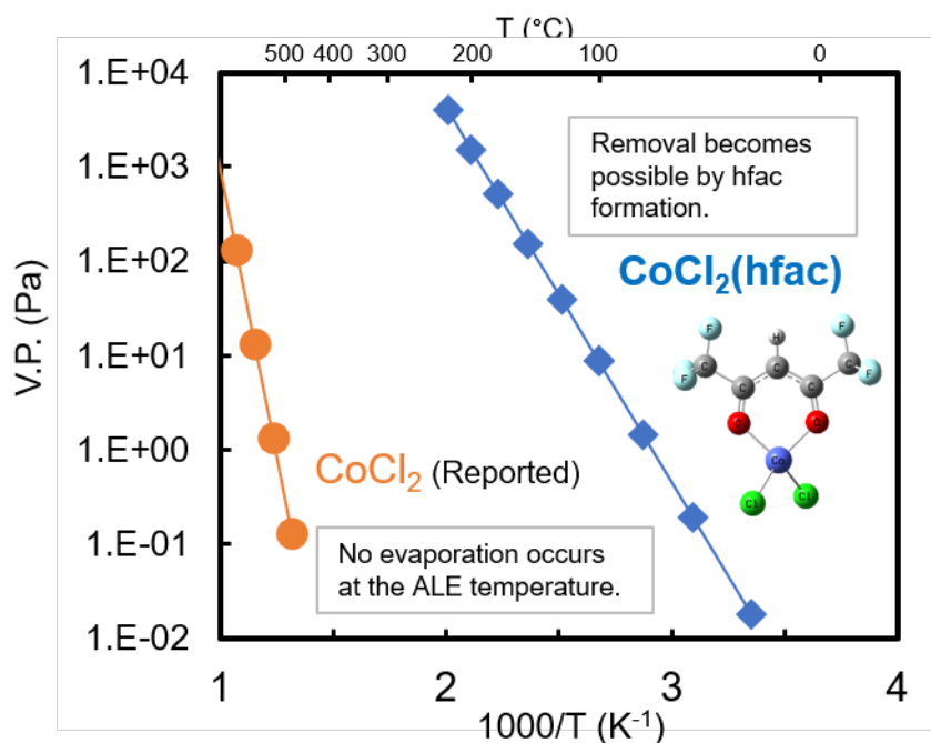
Fig.2 Estimation of volatile chemical compounds for Co-ALE. The chlorinated Co surface species evaporates by reacting with Hfac to form a volatile compound.
