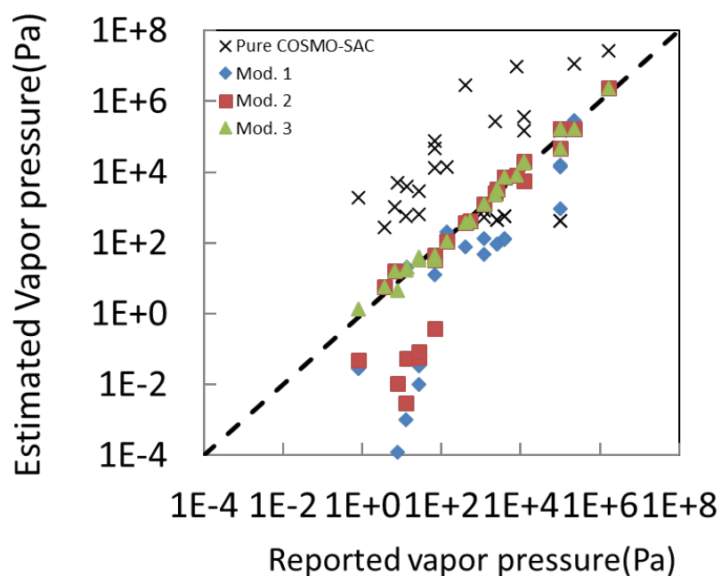
Fig.1 Vapor Pressure estimation of metal containing precursors for ALD/CVD. Several modifications made the accurate estimation.
