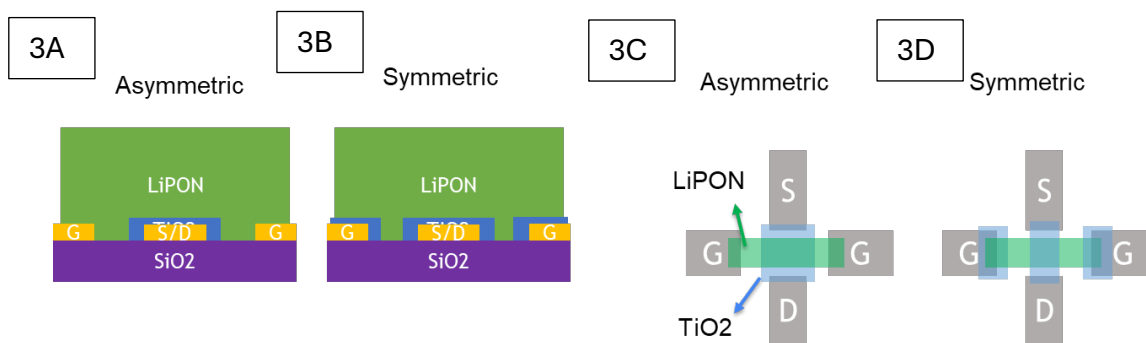
Figure 3: A lateral asymmetric device cross section, B lateral symmetric device cross section, C lateral asymmetric device top view, D lateral symmetric device top view
