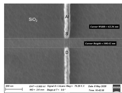
Figure 2: Source and drain fine line lithography for vertical device
