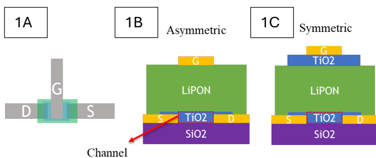
Figure 1: A vertical device top view, B vertical asymmetric cross section, C vertical symmetric cross section
