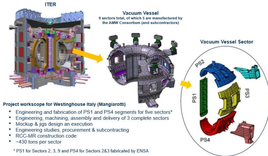
Figure 1: Schematic of ITER Vacuum Vessel, detail on Sectors' configuration and summary of Westinghouse Italy's scope
