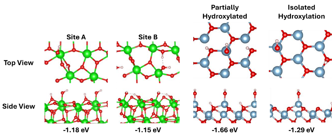
Figure 1: Top and side view of different hydroxyl surface sites on zirconia (left) and alumina (right). Single water adsorption energy informed at the bottom.
