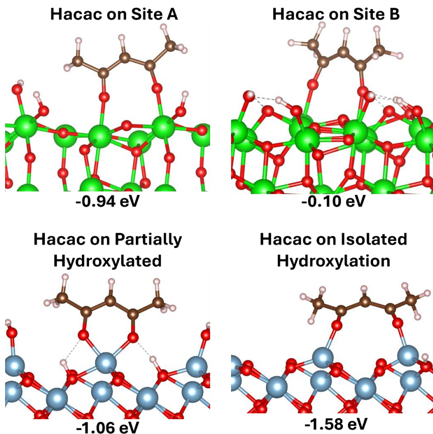
Figure 2: Side views of Hacac inhibitor adsorbed on different sites of zirconia (up) and alumina (bottom).
