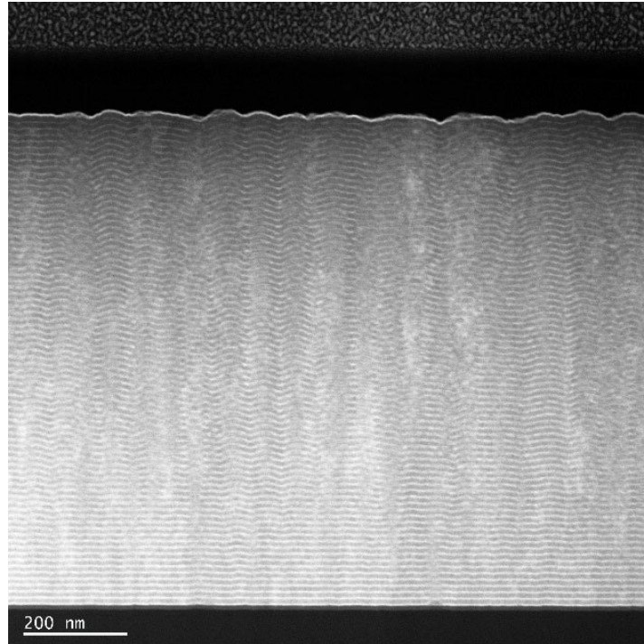
Figure 1: Transmission Electron Microscope image of a (\text{Fe}_{50}\text{Co}_{50}\text{-Ag})_{\times 77} multilayer thin film stack 930 nm thick.
