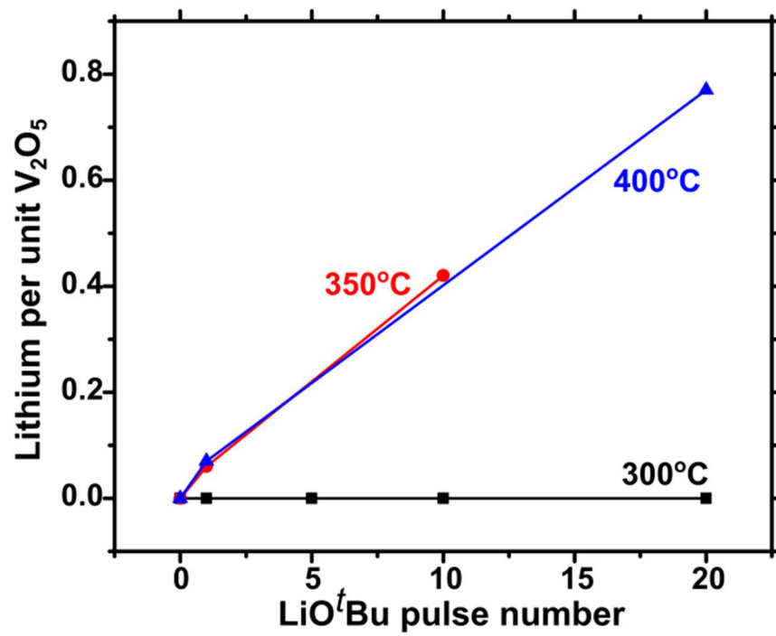
Figure 1: Lithiation state of V 2 O 5 as a function of LiO t Bu pulse number, calculated from electrochemical cycling.
