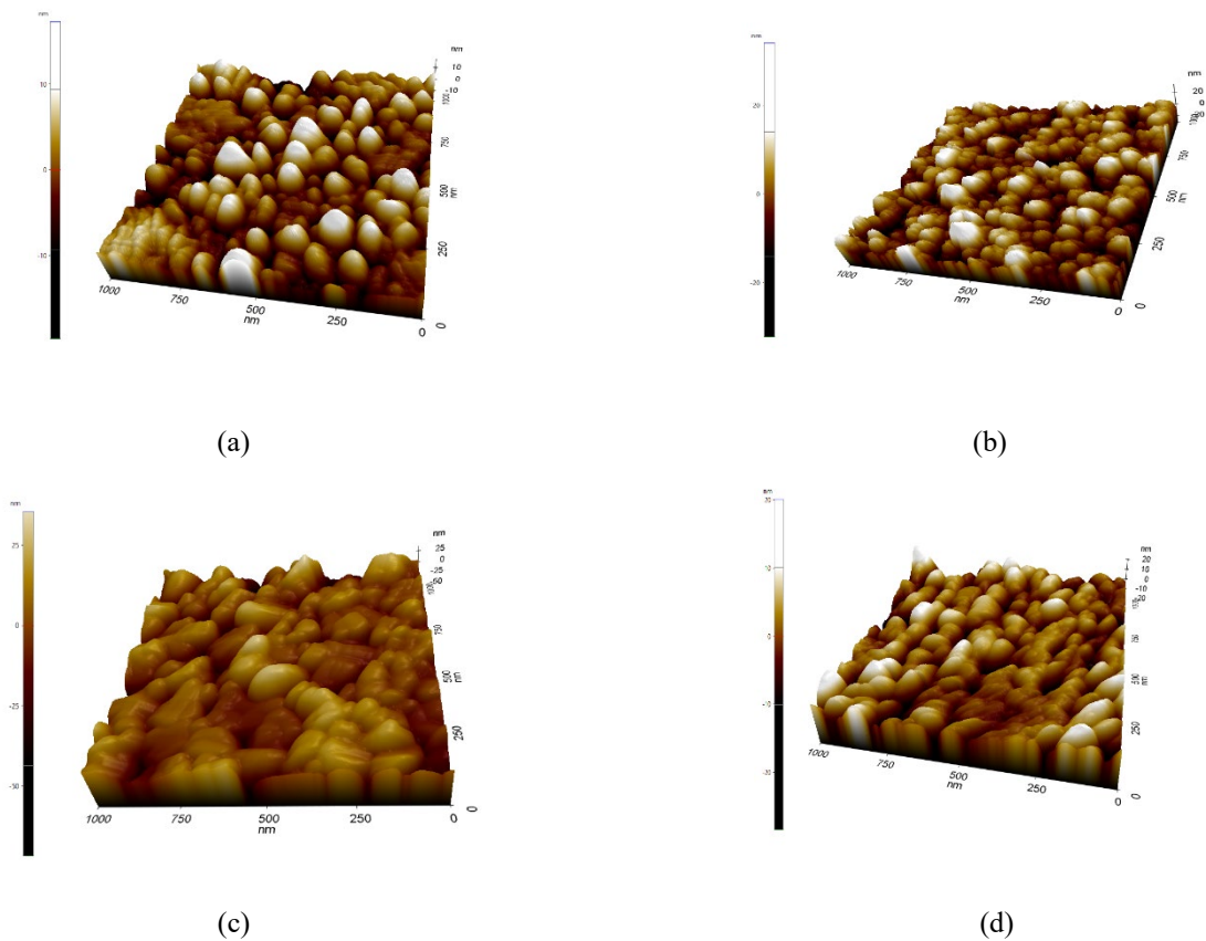
Fig. 2: AFM images of (a) \text{NaNbO}_3 and effect of doping 1 mol% of (b) Fe, (c) Ni and (d) Cu into Nb site of \text{ABO}_3 perovskite. The grain size was measured to be (a) 65-70 nm, (b) 50-60 nm, (c) 87-120 nm, and (d) 80 nm respectively.
