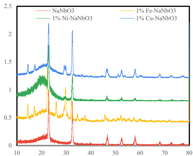
Fig. 1: XRD patterns of pure \text{NaNbO}_3 and doped with 1 mol % Fe, Ni and Cu.
