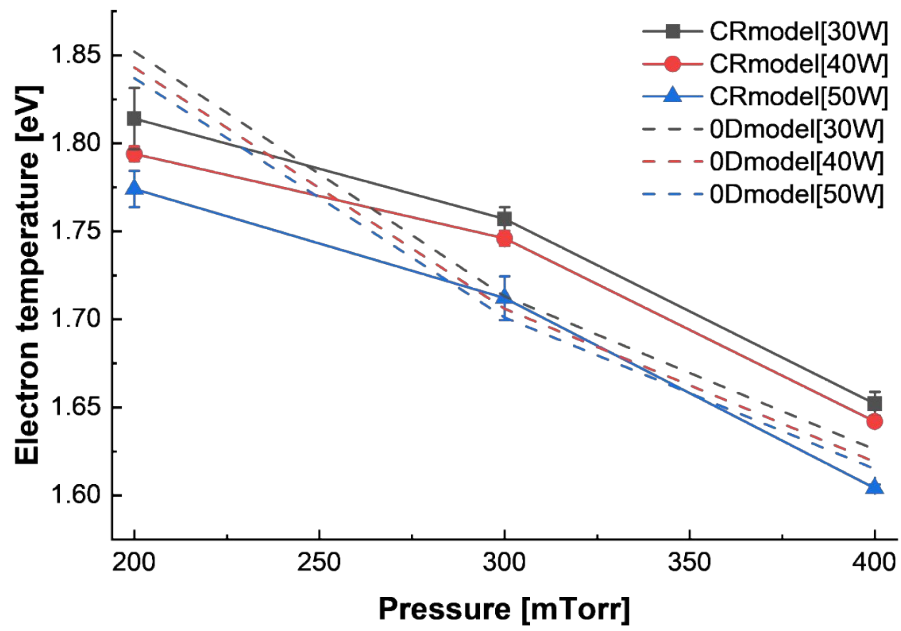
Fig1. Comparison of Electron Temperature Obtained from the 0D Model and CR-OES Inversion
