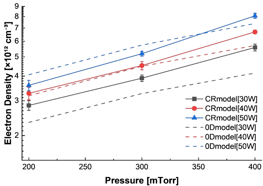
Fig2. Comparison of Electron Density Obtained from the 0D Model and CR-OES Inversion
