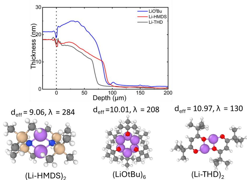
Fig. 1. Li-TP conformality dependence on precursor oligomeric structure: Imaging-ellipsometry assisted thickness profiles for Li-TP deposited on LHAR test structures with 50 ALD/MLD cycles (top). The stable oligomers from each precursor, along with the effective diameter ( d_{\text{eff}} , Å) and mean free paths (MFP, \lambda , nm), are provided in the lower section.
